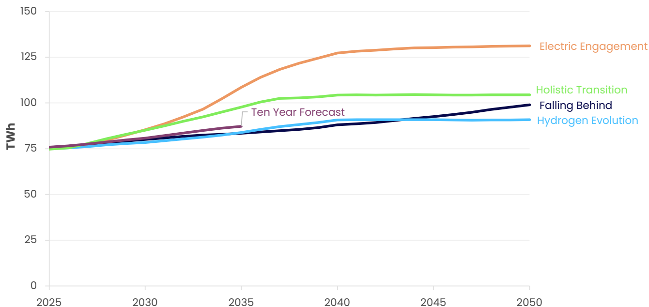
52. Industrial electricity demand (excluding hydrogen production)
