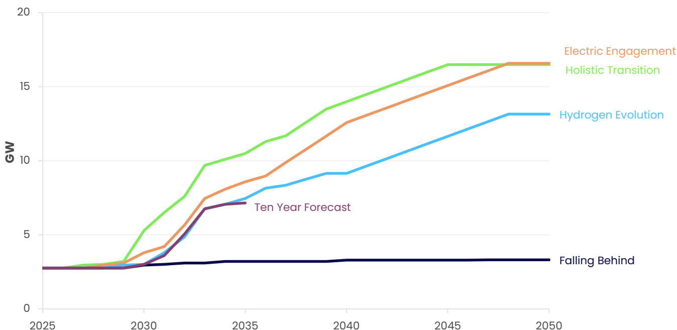
62. Long-duration energy storage installed capacity (excluding electric vehicles and hydrogen)
